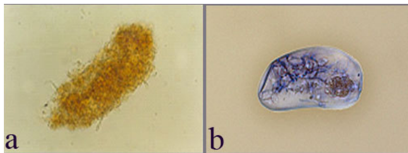
Fig. 2- Immature eggs of Heterodera schachtii infected by fungi; a: C. destructans var. crassum (400×); b: P. lilacinus (400 ×)
